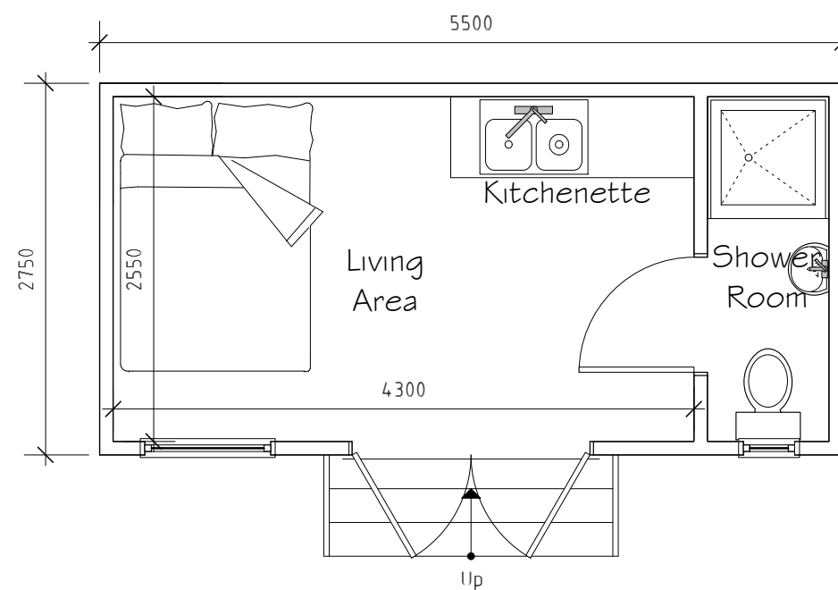
Floor Plan 1:50
