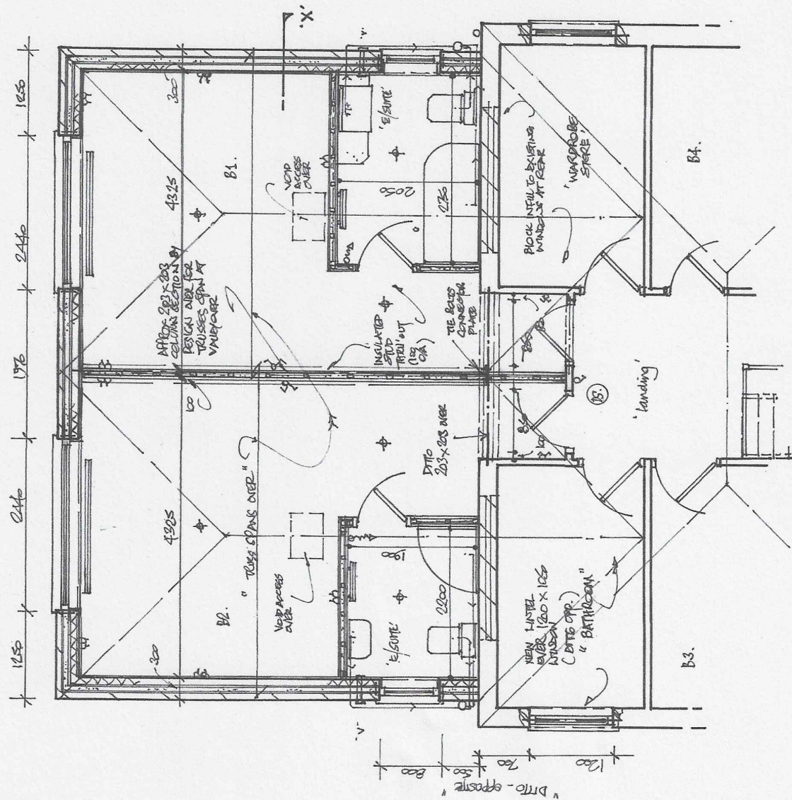
"AS PROPOSED" FIRST FLOOR AT REAR 1:50
