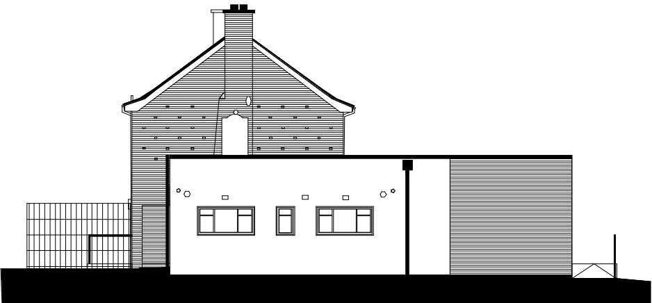
CONSENTED NORTH (SIDE) ELEVATION
