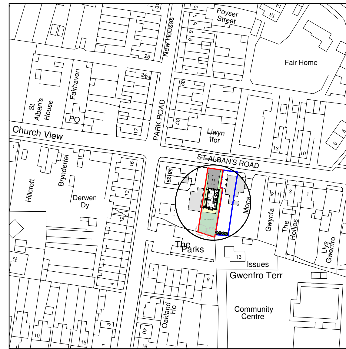
Location Plan 1:1250
