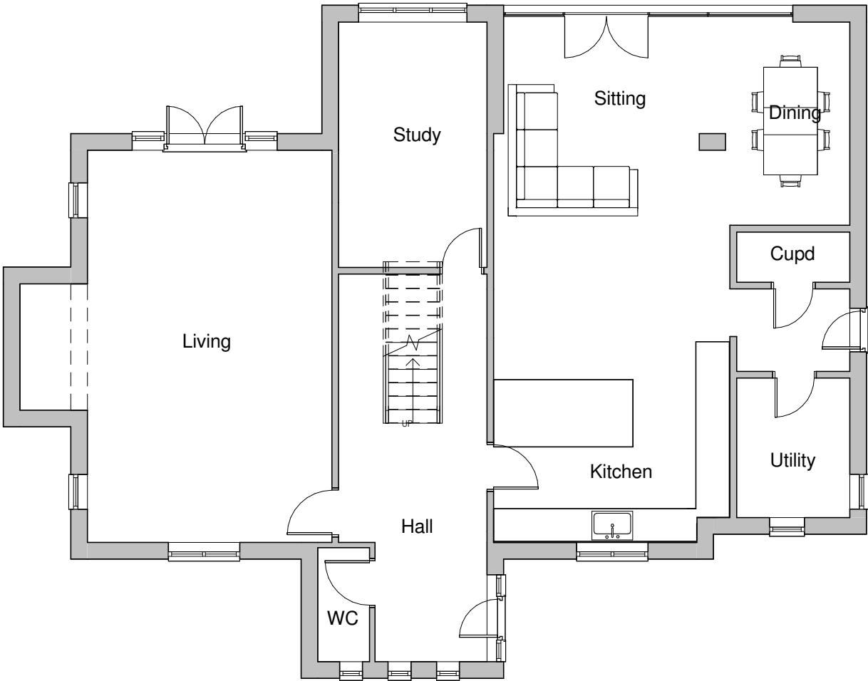
Ground Floor 1 : 100
