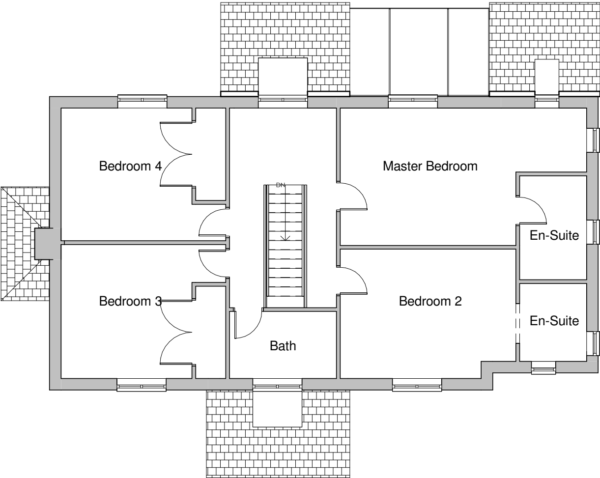
First Floor 1 : 100
