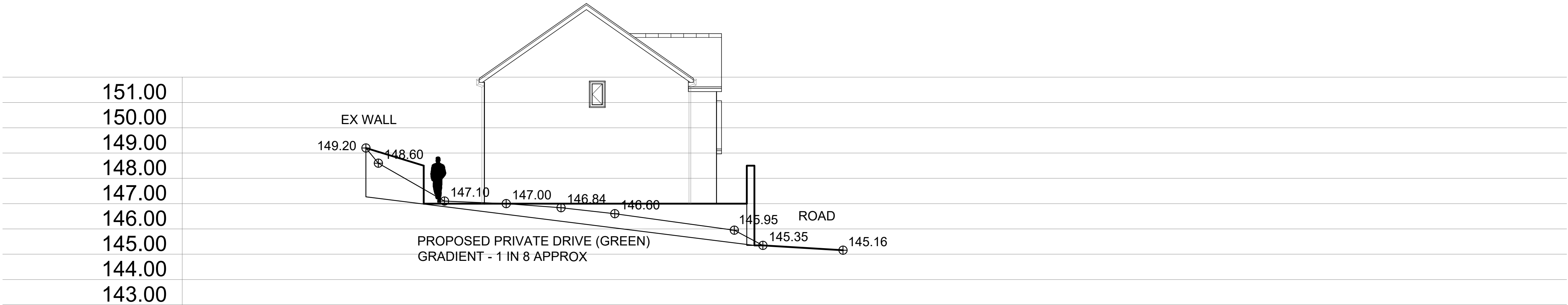
Section C-C as Proposed
