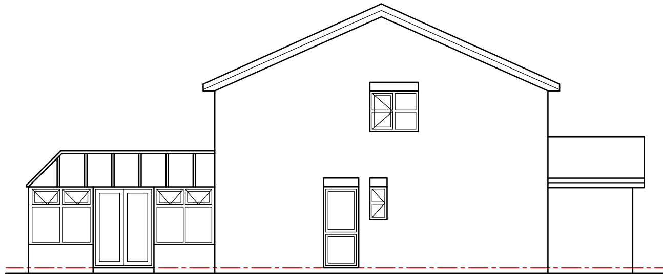
Side Elevation
