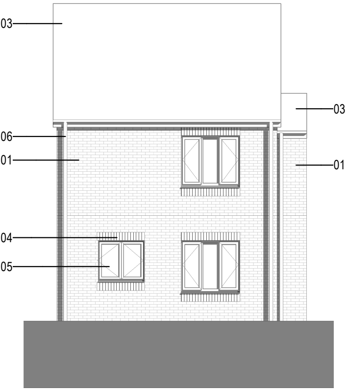
Rear Elevation 1 : 100
