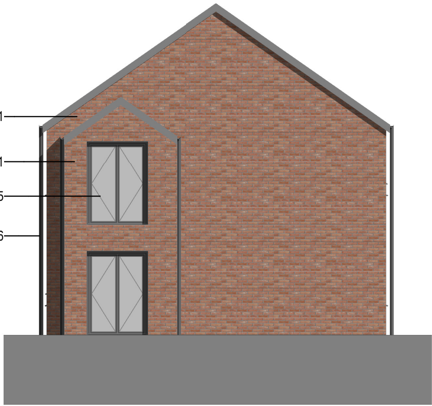
Side Elevation 1 : 100
