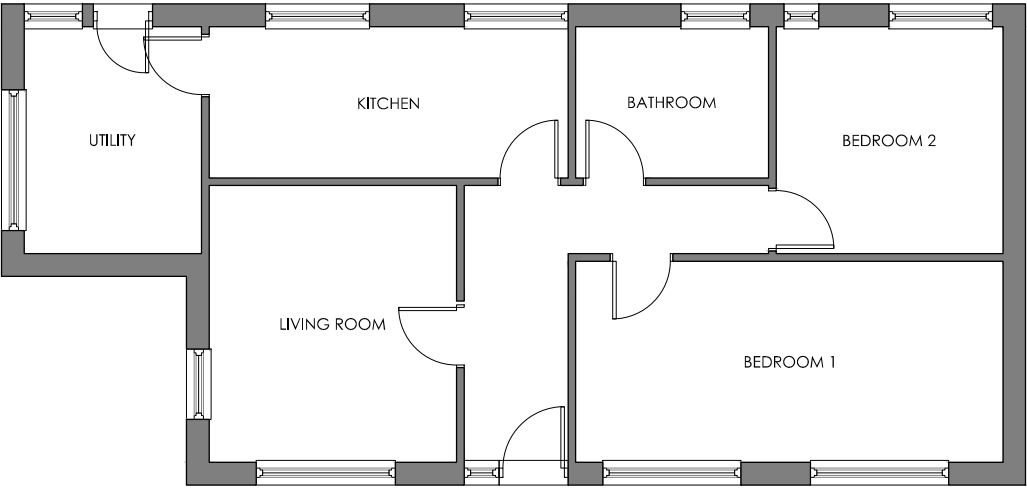
EXISTING FLOOR PLANS (1:100)
