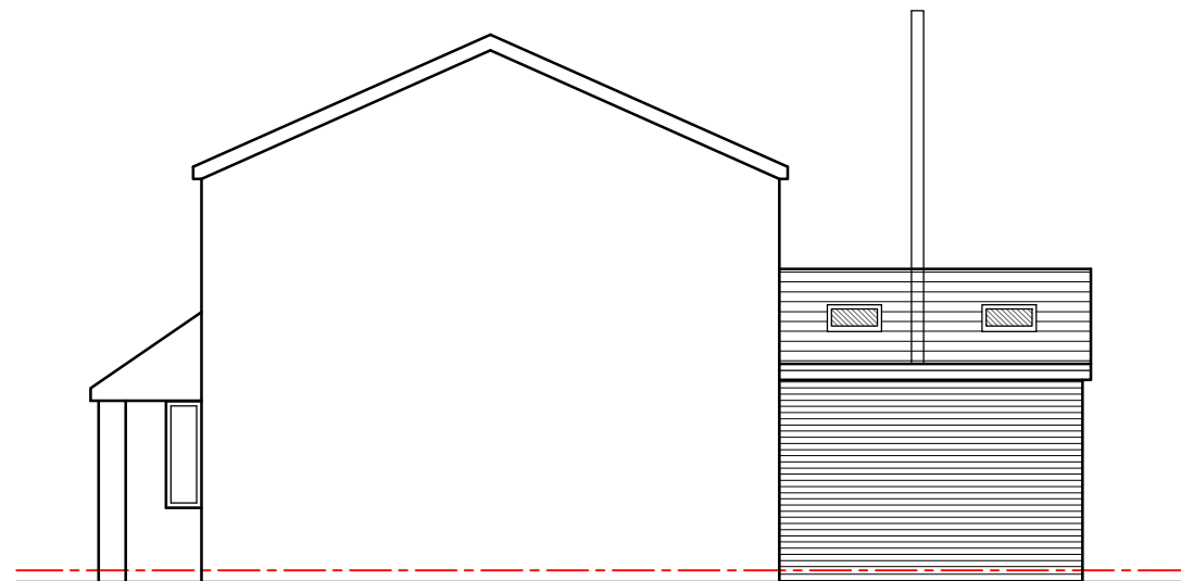
Side 01 Elevation
