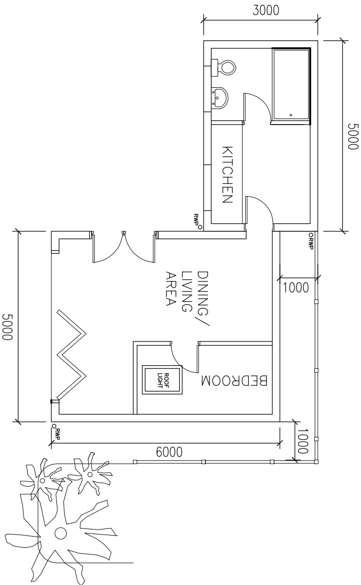
FLOOR PLAN
