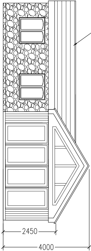
WEST ELEVATION CANALSIDE
