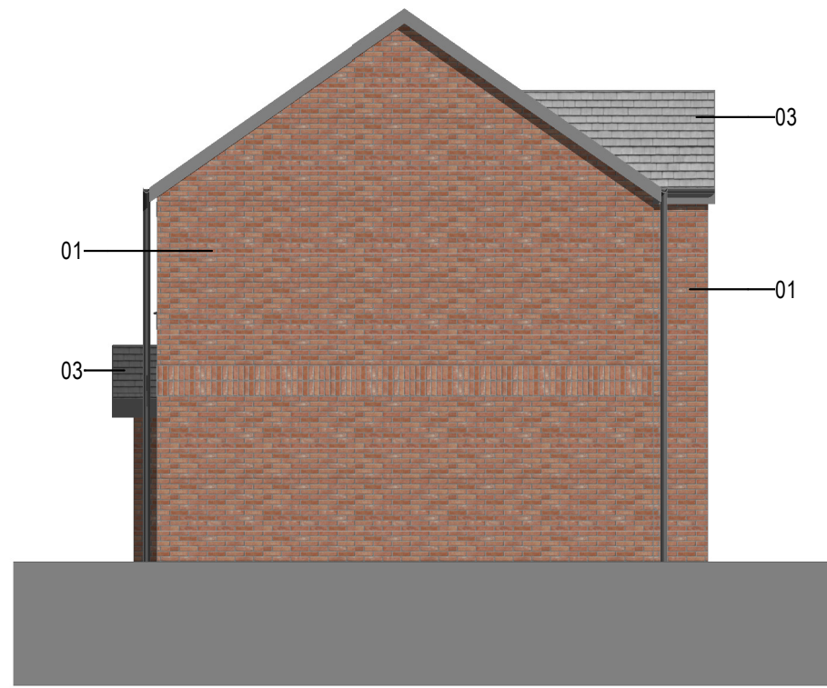
Side Elevation 1 : 100
