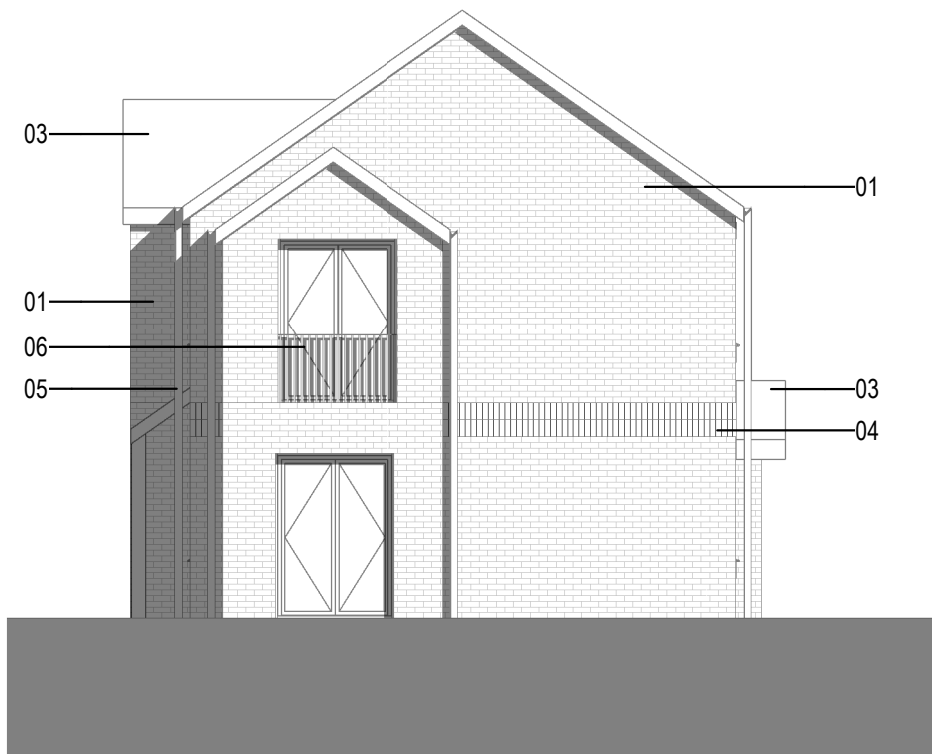
Side Elevation 1 : 100
