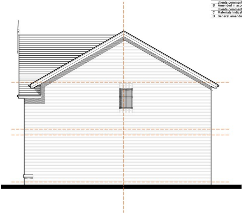
SIDE ELEVATION (RIGHT)
