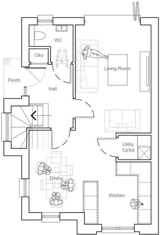
GROUND FLOOR TYPE F 47.6 sqm
