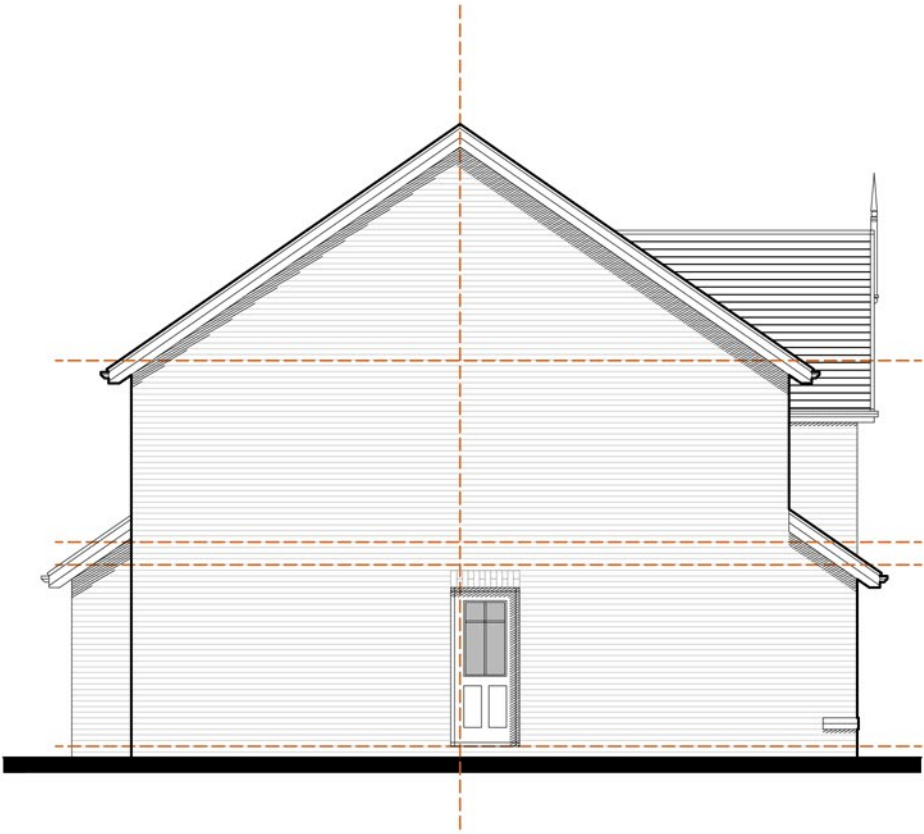
SIDE ELEVATION (LEFT)
