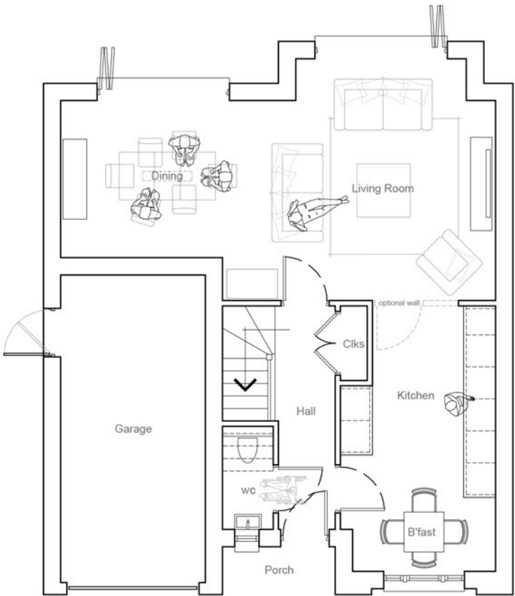
GROUND FLOOR TYPE E 54.85 sqm
