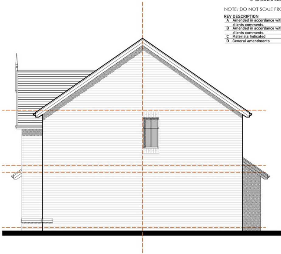
SIDE ELEVATION (RIGHT)
