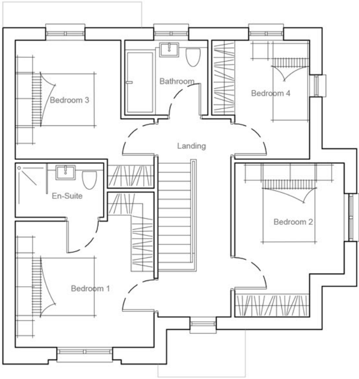
FIRST FLOOR TYPE A 60.75sqm
