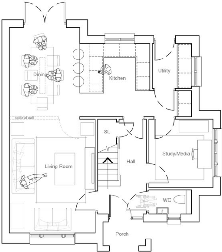
GROUND FLOOR TYPE A 62.75sqm
