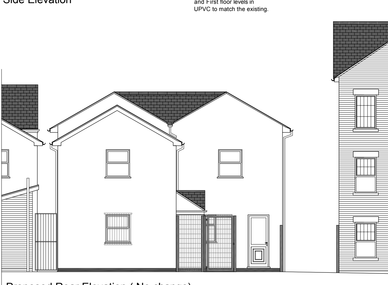
Proposed Rear Elevation ( No change)
