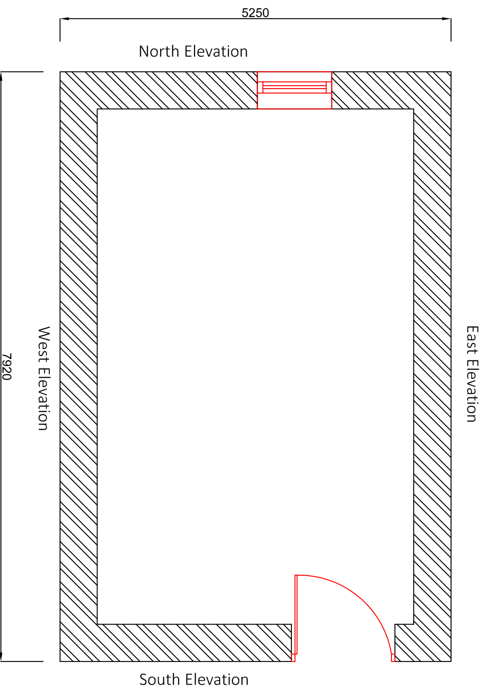
GROUND FLOOR PLAN Scale 1 / 50
