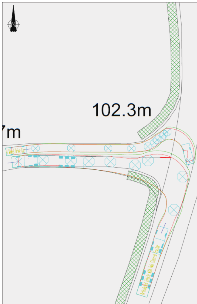
Swept path diagrams
