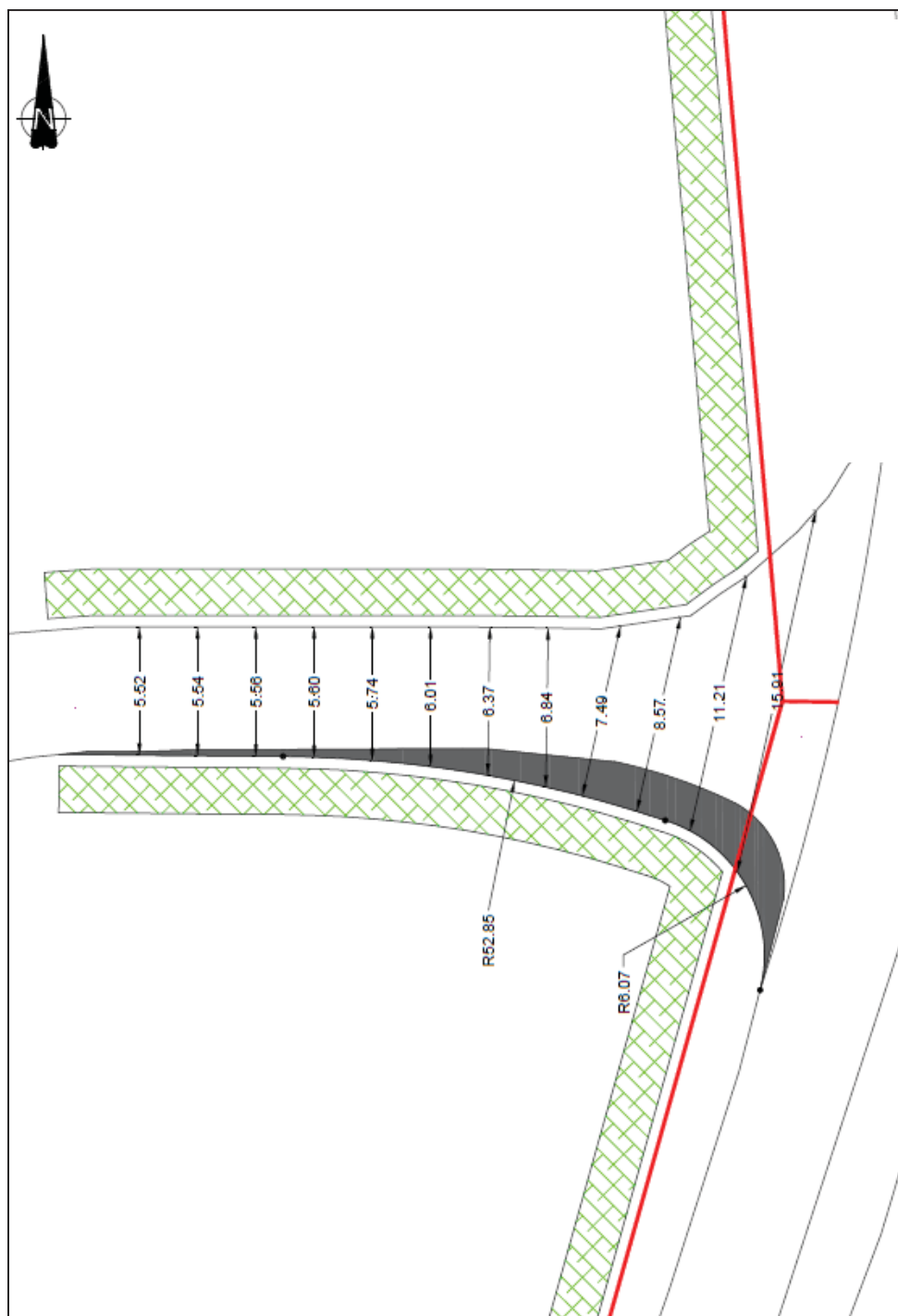
Proposed junction widening (shown shaded)
