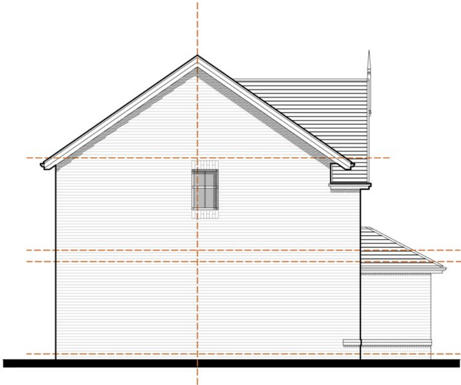
SIDE ELEVATION (LEFT)
