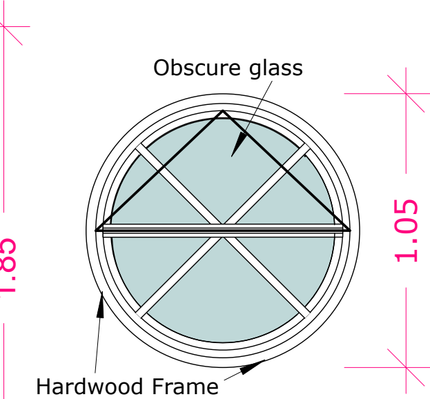
SW Elev. Window 1-20
