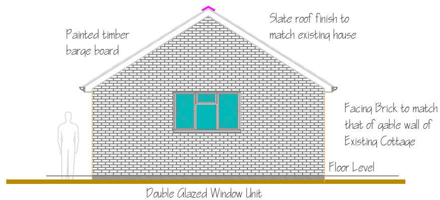
PROPOSED GABLE ELEVATION A SCALE 1:100
