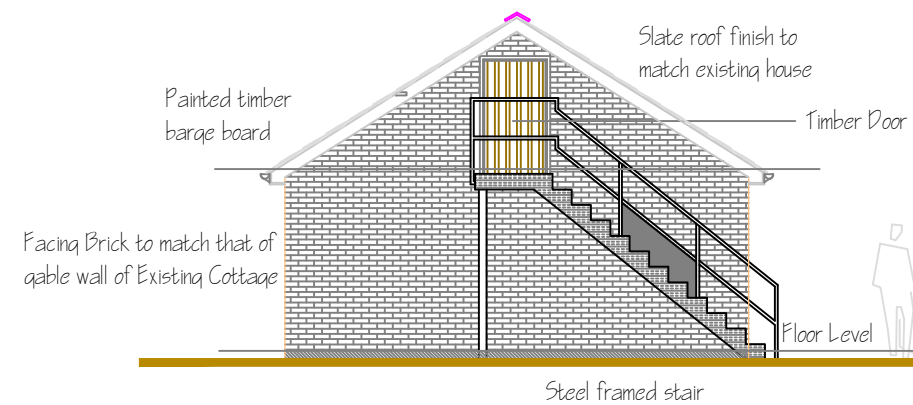
PROPOSED GABLE ELEVATION B SCALE 1:100
