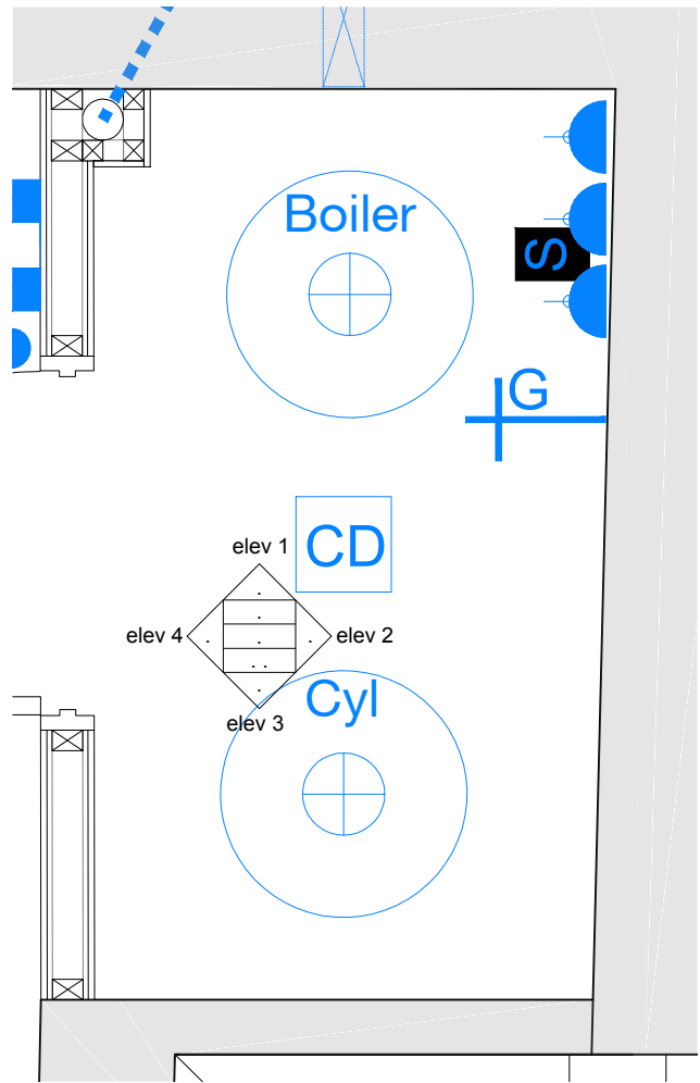
GROUND FLOOR BOILER ROOM PLAN
