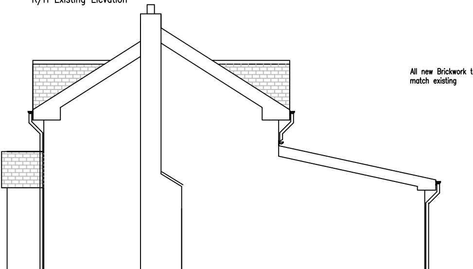
R/H Existing Elevation
