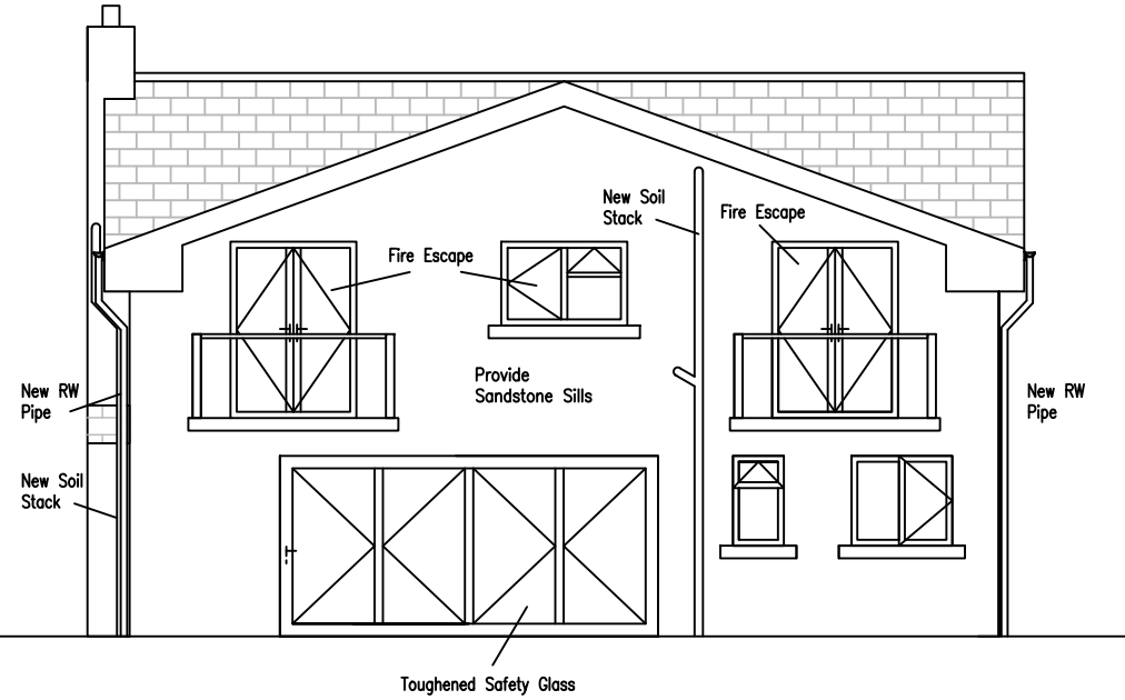
Rear Proposed Elevation
