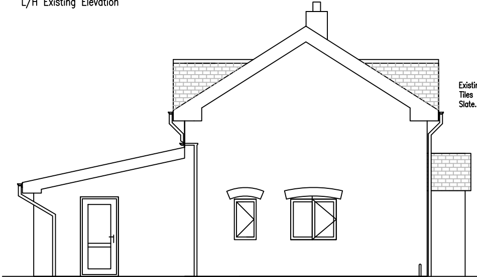
L/H Existing Elevation
