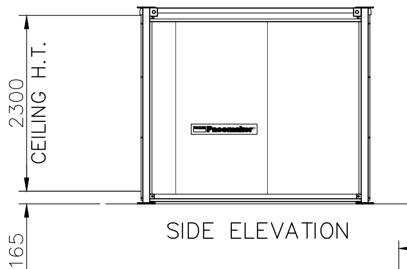
SIDE ELEVATION
