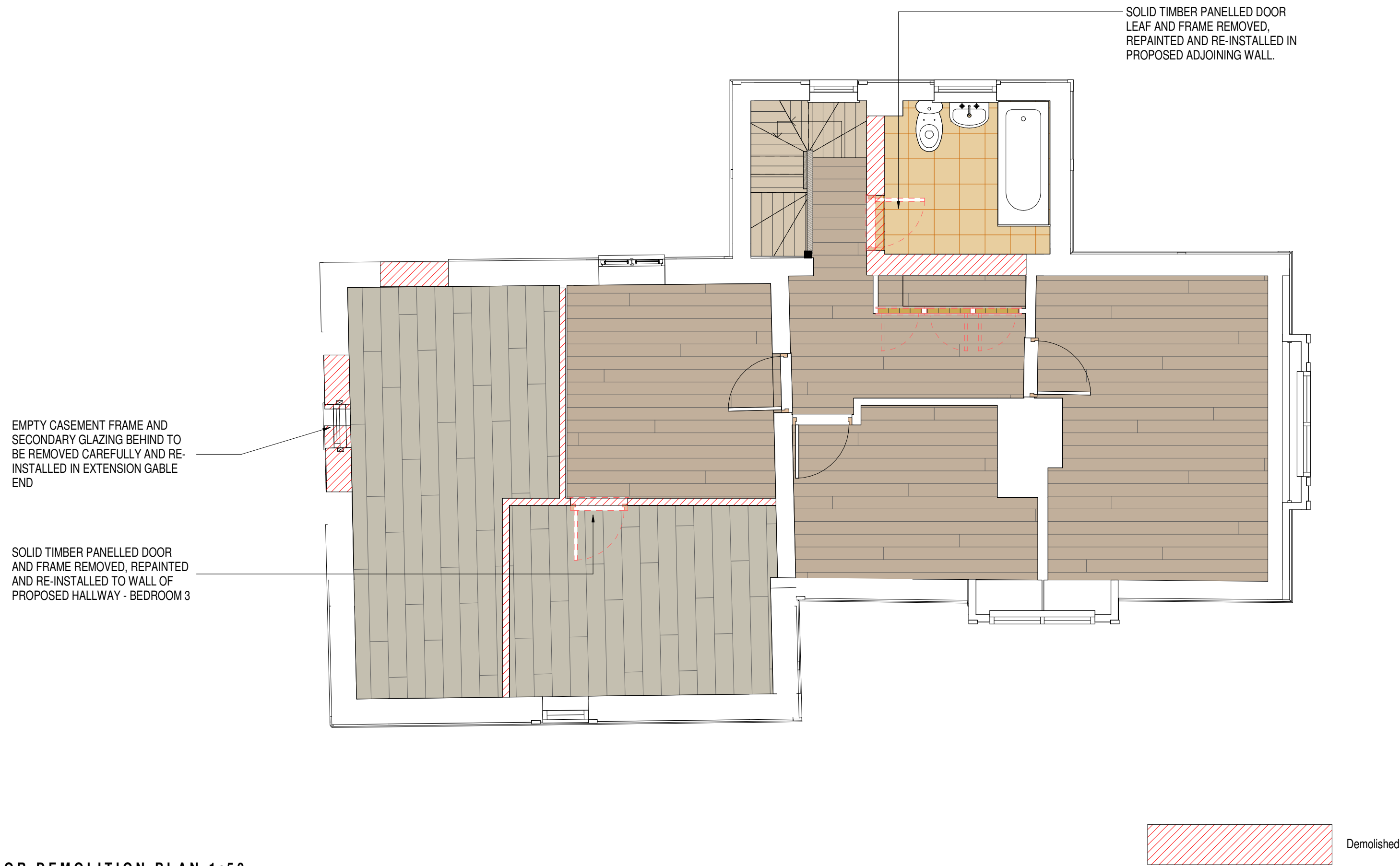
FIRST FLOOR DEMOLITION PLAN 1:50
