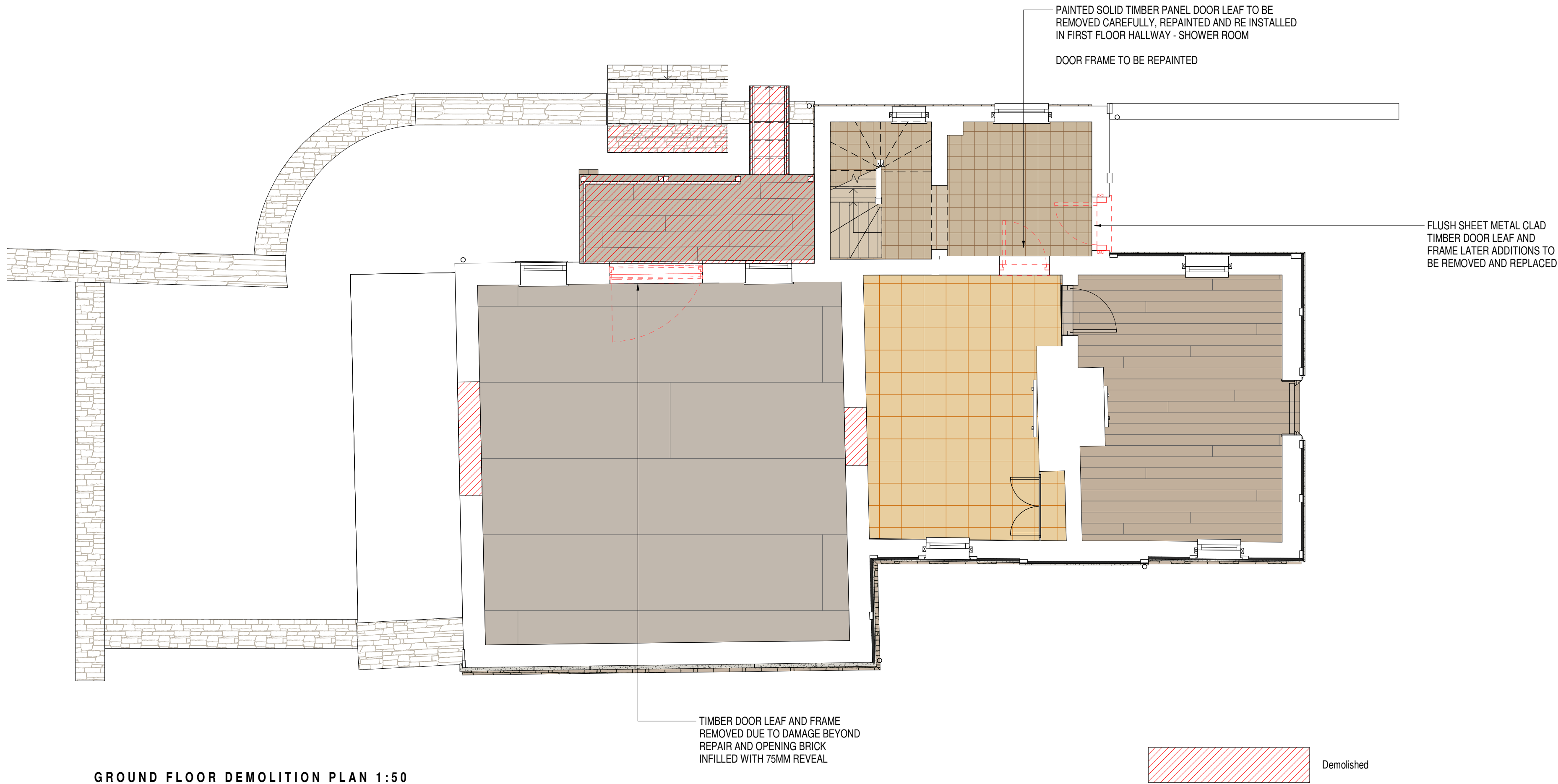
GROUND FLOOR DEMOLITION PLAN 1:50
