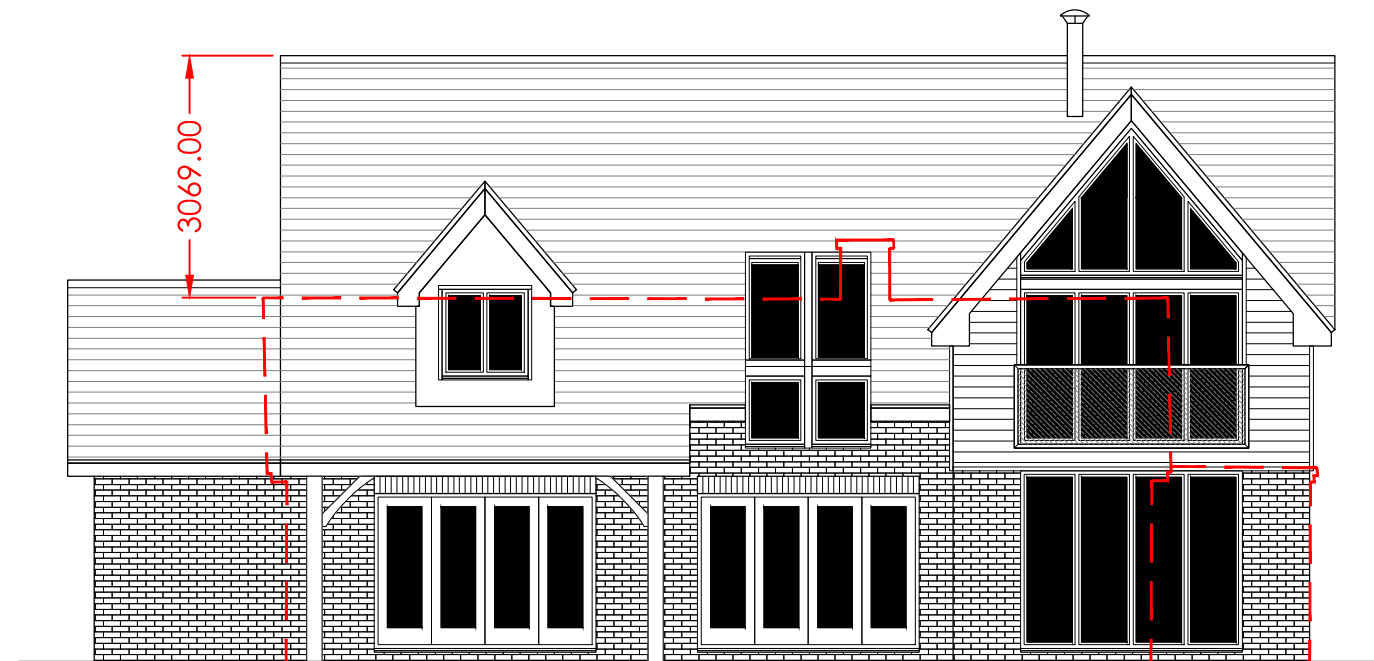
REAR ELEVATION
