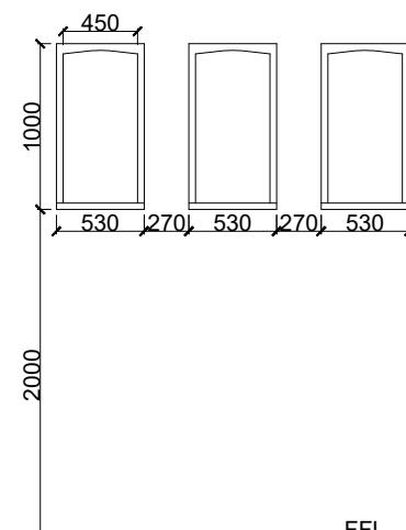
3 No. EXISTING HIGH LEVEL WINDOW (internal configuration)
