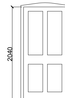
EXTERNAL FRAME DOOR Details of s/w rails, styles, panels, central mullions & beads to be checked on site based on Gents toilets. Frame made of s/w to fit opening. Decorate to match existing panel doors along the platform.
