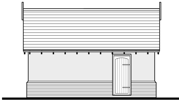
Proposed Side Elevation View H - 1:100
