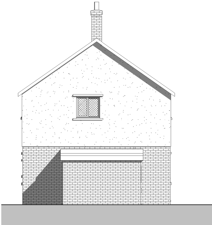
Side Elevation 1 : 100
