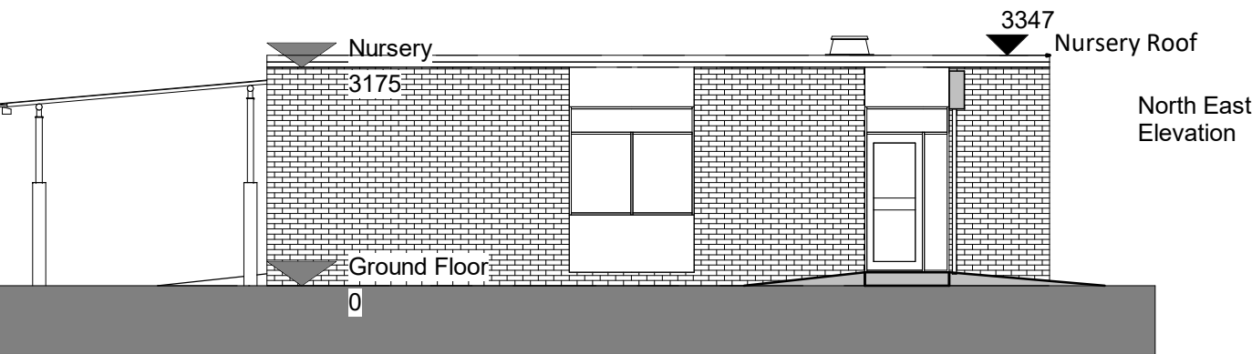
PL - Proposed North East Nursery Elevation 1 : 100
