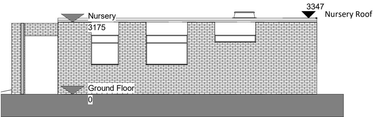
PL - Proposed North West Nursery Elevation 1 : 100
