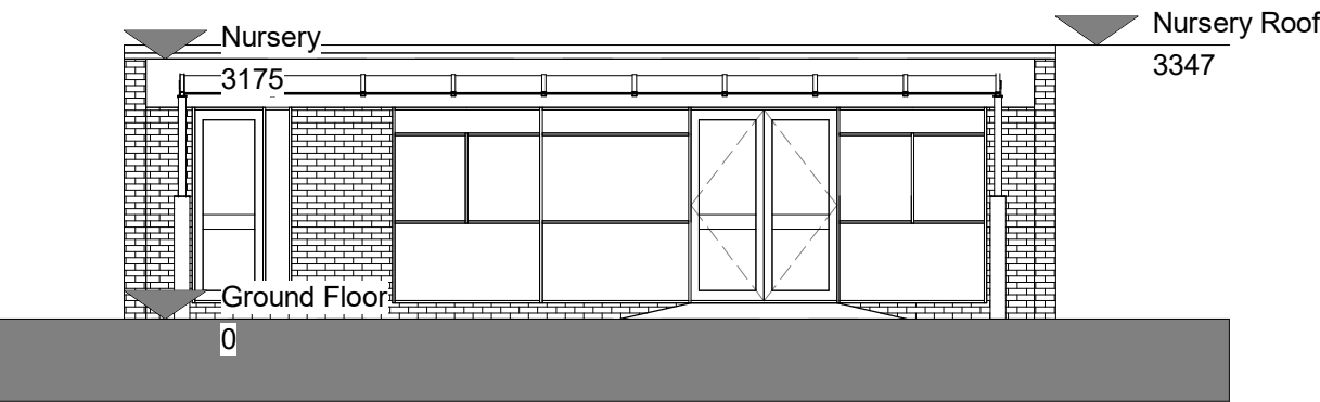
PL - Proposed South East Nursery Elevation 1 : 100
