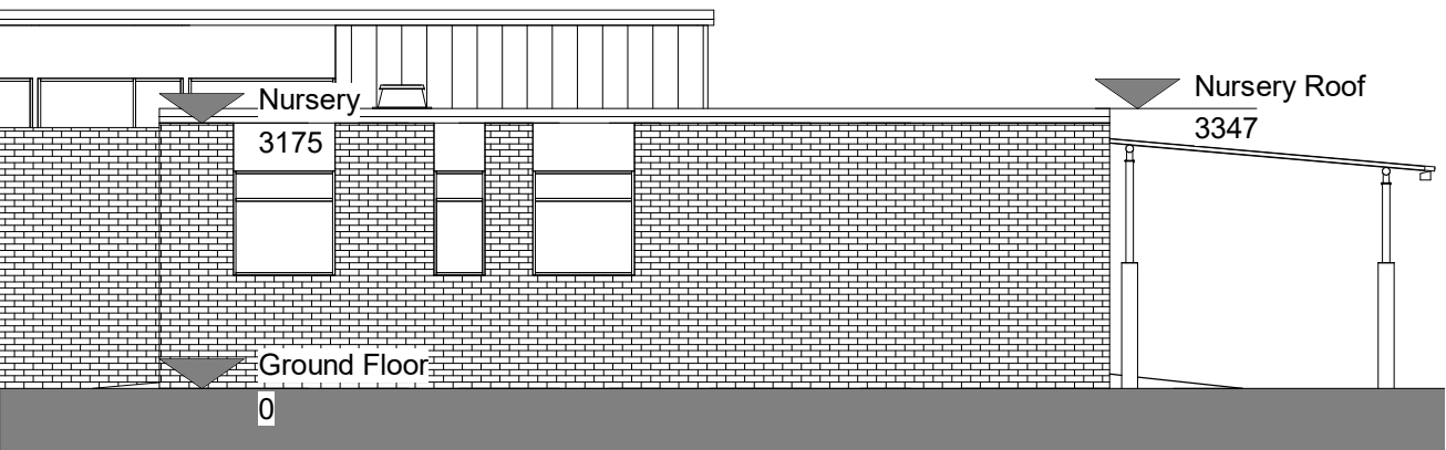
PL - Proposed South West Nursery Elevation 1 : 100
