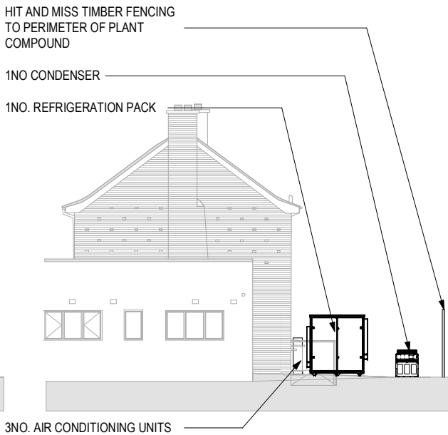
PROPOSED SOUTH (SIDE) ELEVATION (FENCE OMITTED)
