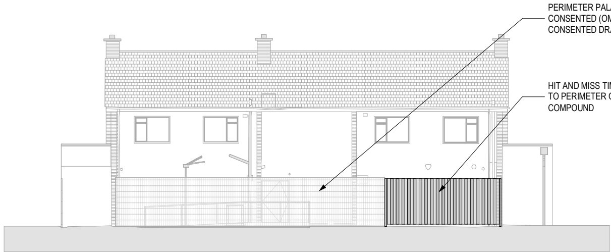
PROPOSED EAST (REAR) ELEVATION
