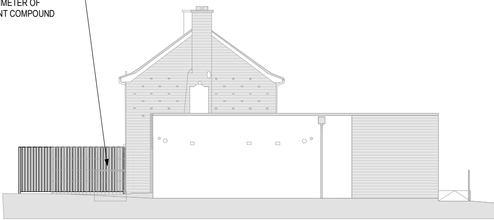
PROPOSED NORTH (SIDE) ELEVATION
