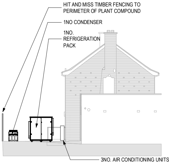
PROPOSED NORTH (SIDE) ELEVATION (FENCE OMITTED)
