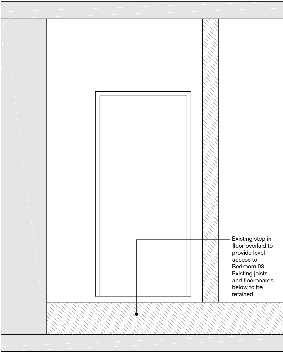
ELEVATION 03
