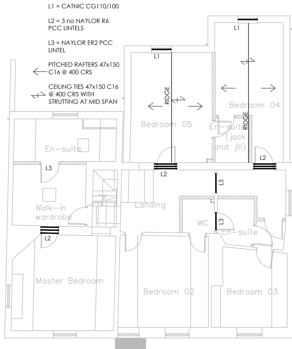
TWO STOREY EXTENSION ROOF AND 1ST FLOOR LINTELS 1:100
