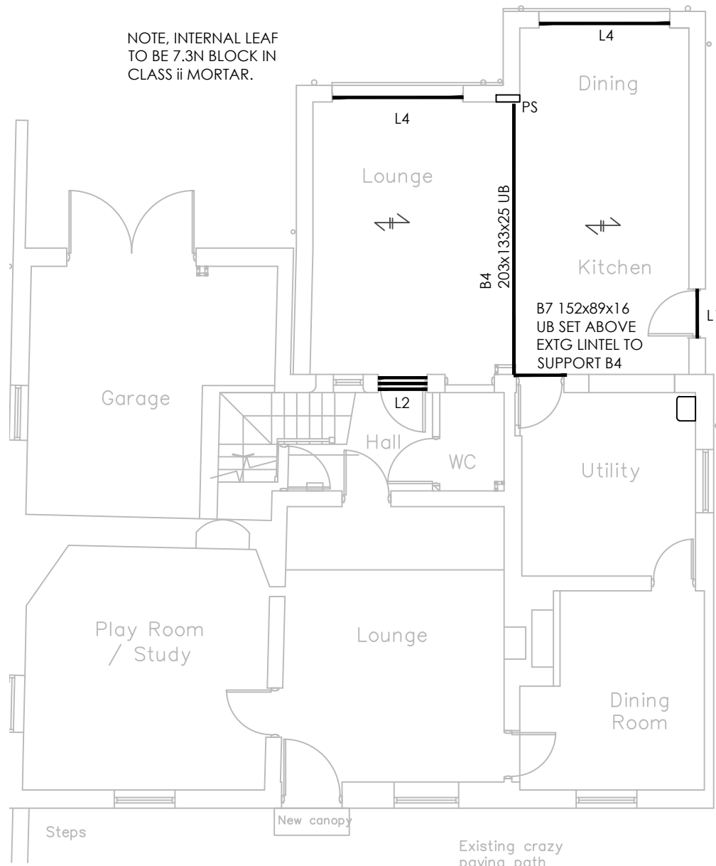
GROUND FLOOR STEELWORK & LINTELS 1:100
