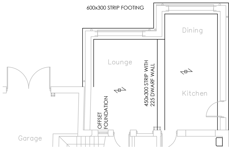
GROUND FLOOR & FOUNDATIONS 1:100
