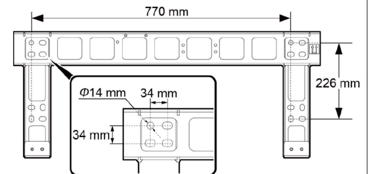
Figure 4-10 Mounting bracket dimensions
