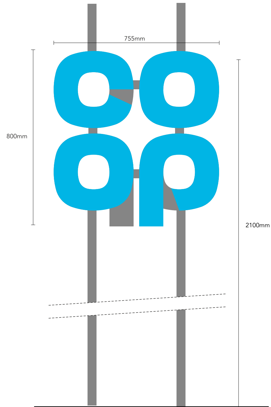
Face view - scale 1:10 @ A3
