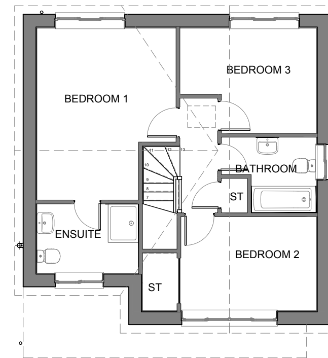
FIRST FLOORPLAN
