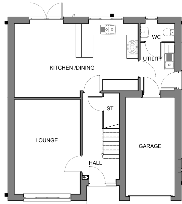
GROUND FLOORPLAN
