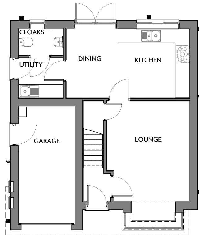
GROUND FLOORPLAN
