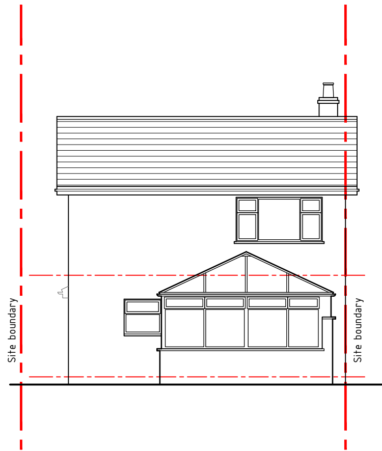
Rear Elevation 1:100
