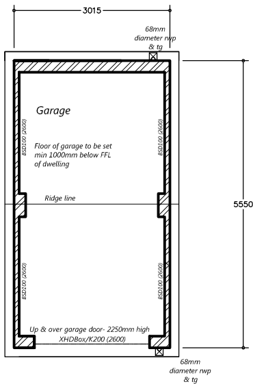
Floor Layout Plan single
