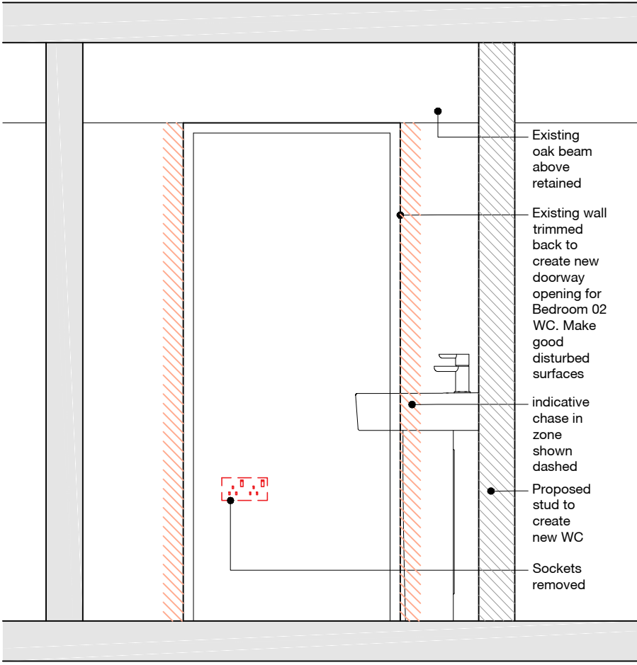
ELEVATION 03
