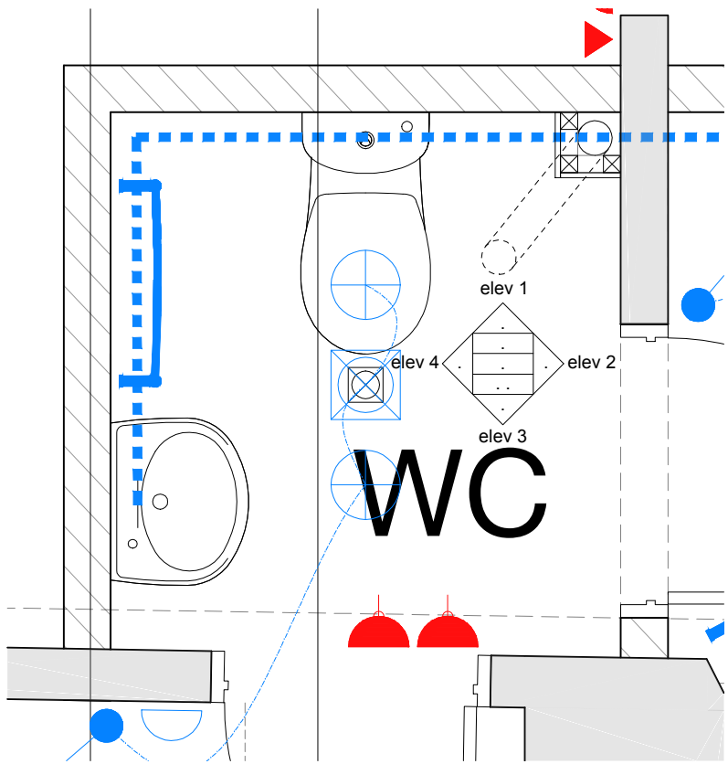
FIRST FLOOR WC PLAN
