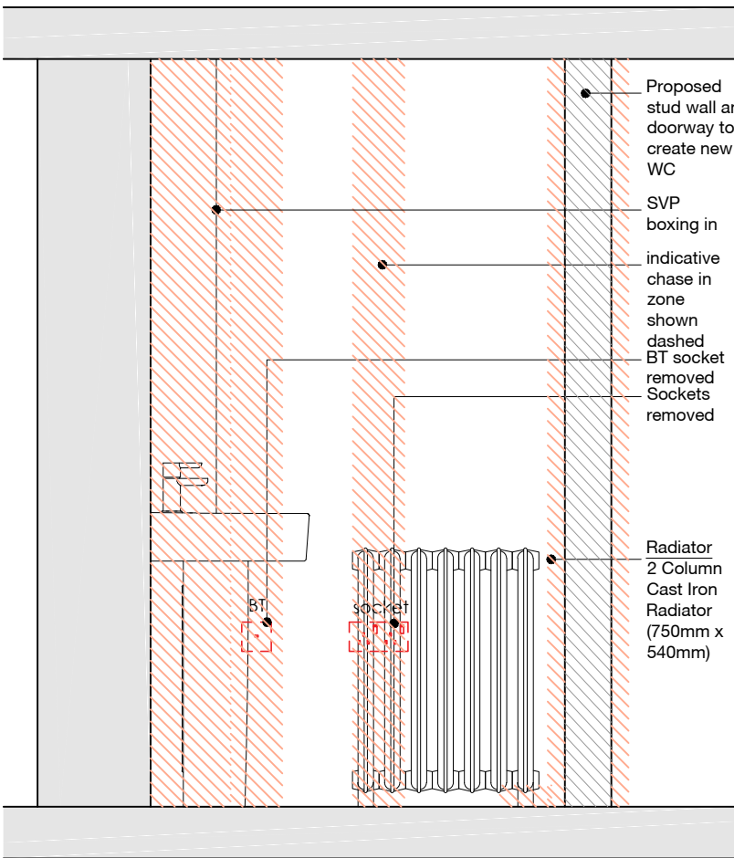
ELEVATION 03
