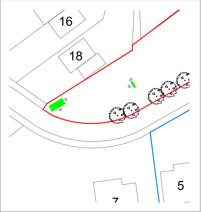
Orientation Plan Scale 1:500
