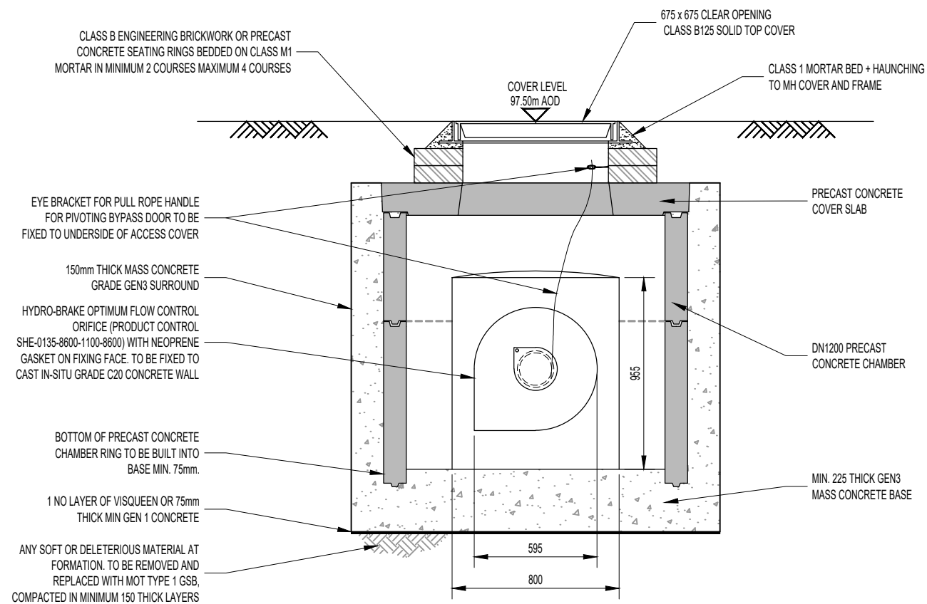
SECTION A
