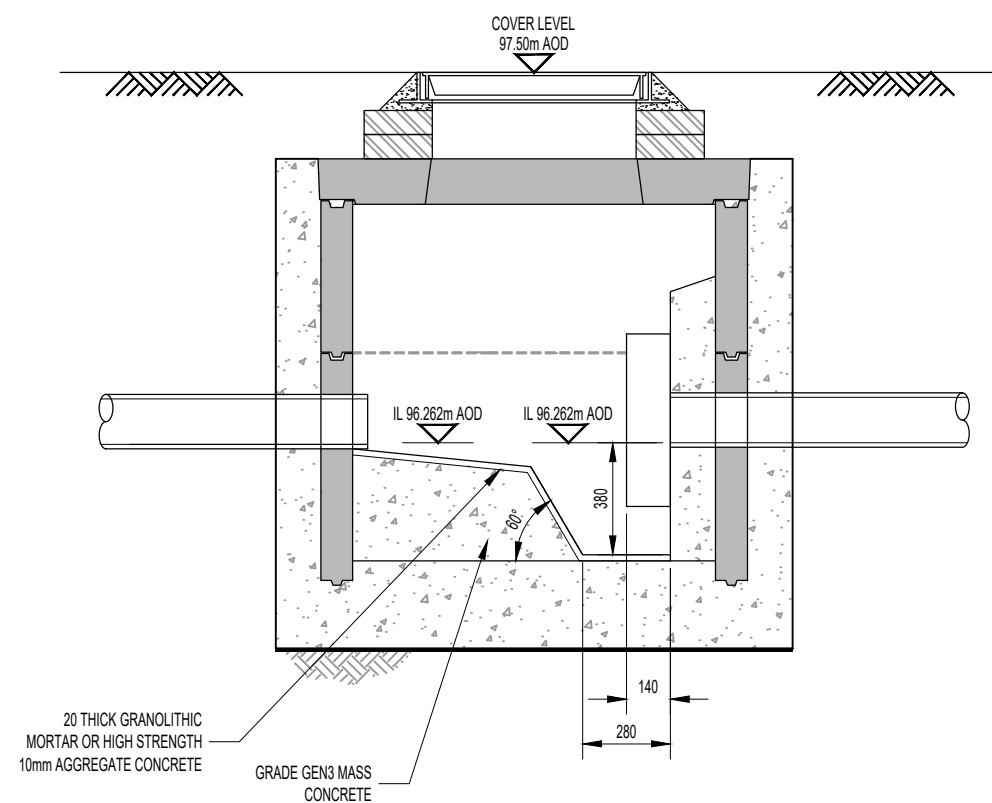
SECTION B
