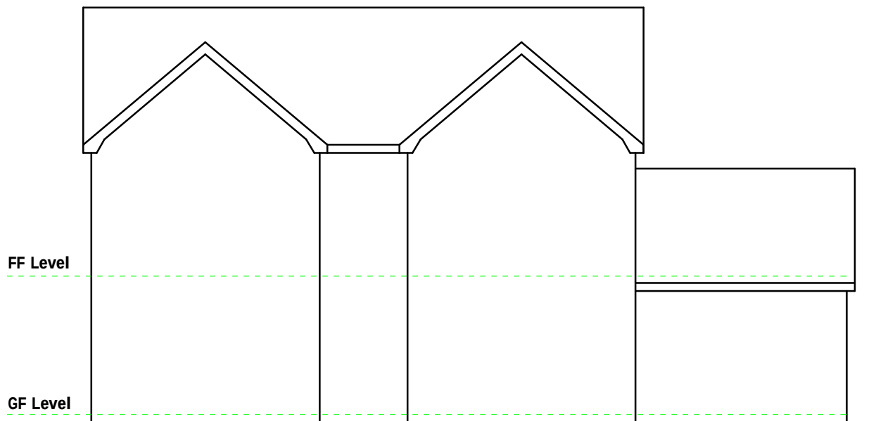
Typical Elevation 1:100
