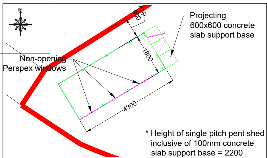
Garden Shed Scale 1:100
