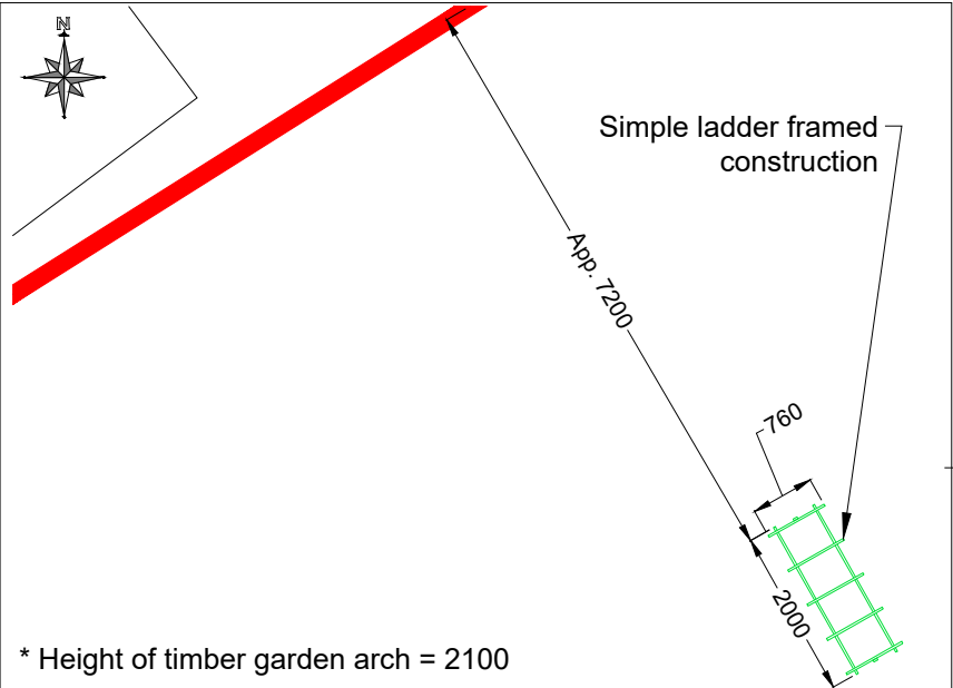
Garden Arch Scale 1:100
