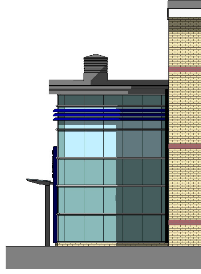
2 Proposed South 1 : 100
