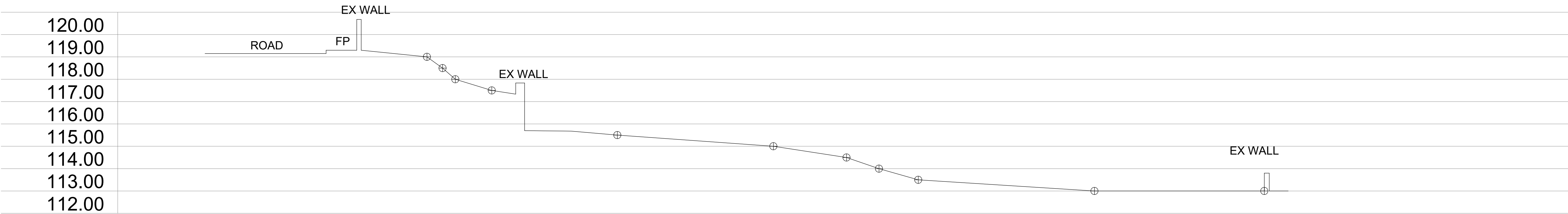
Section A-A as Existing
