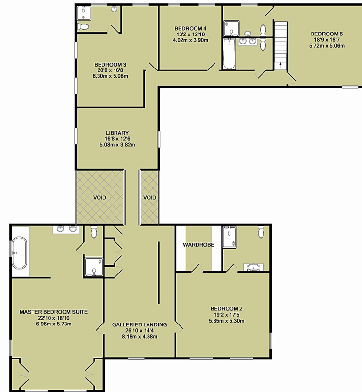
1ST FLOOR
