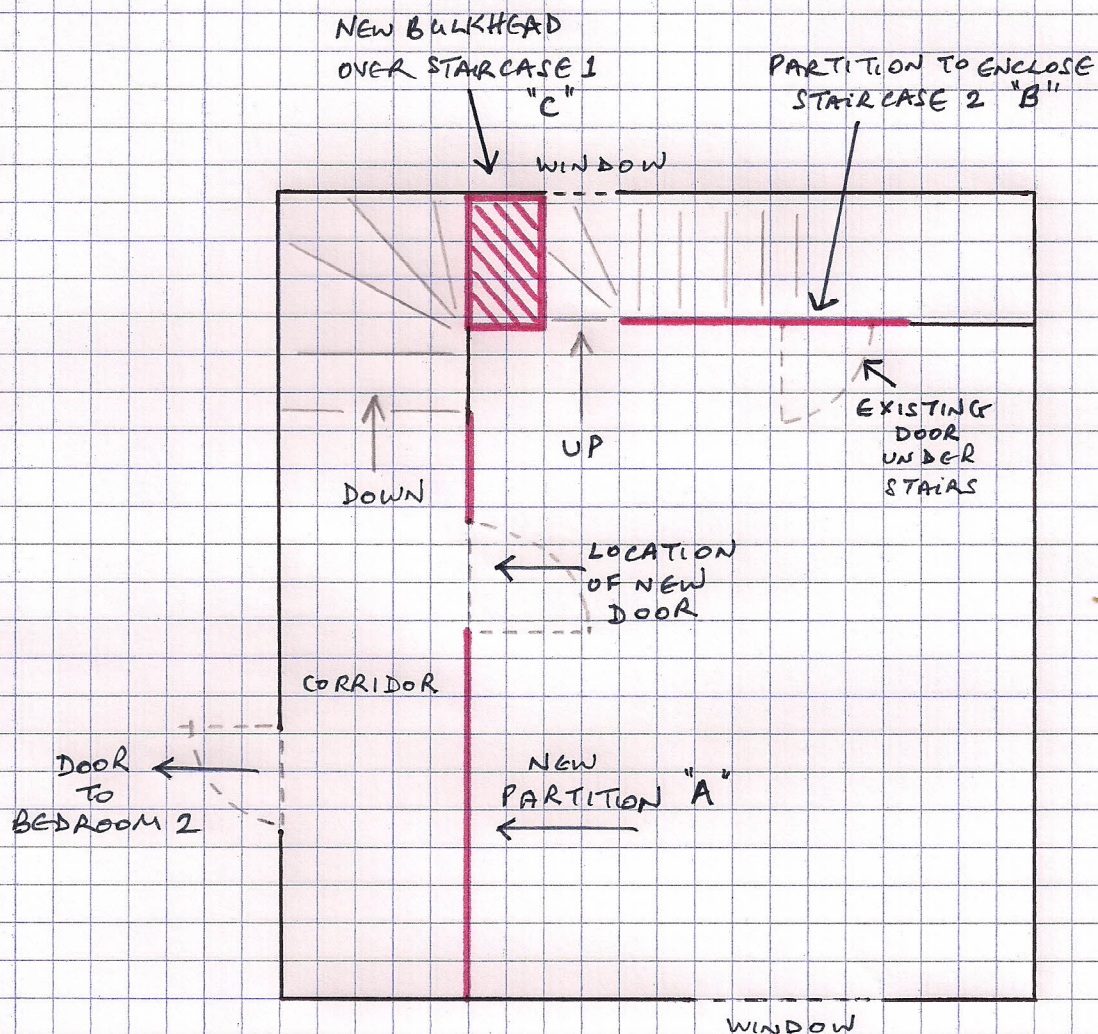
BEDROOM 1 FLOOR PLAN
