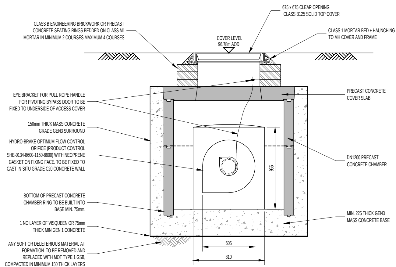
SECTION A
