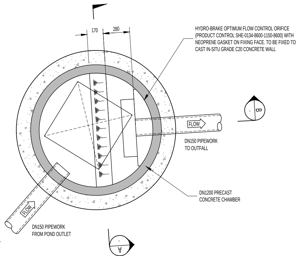
PLAN VIEW
