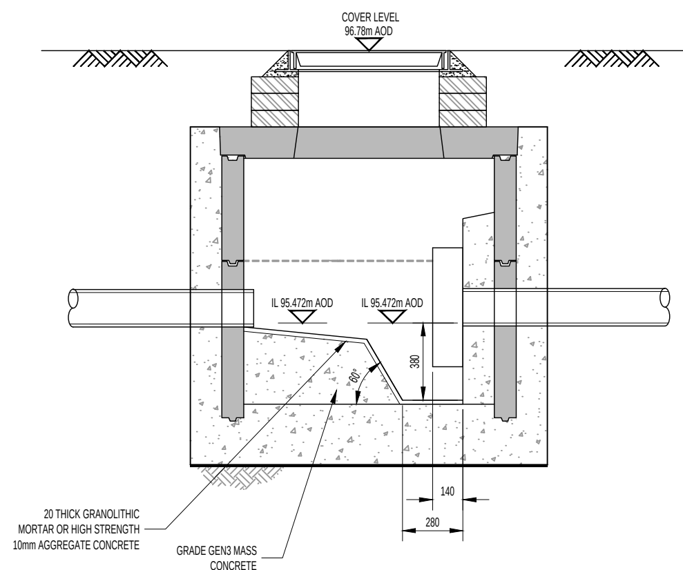
SECTION B
