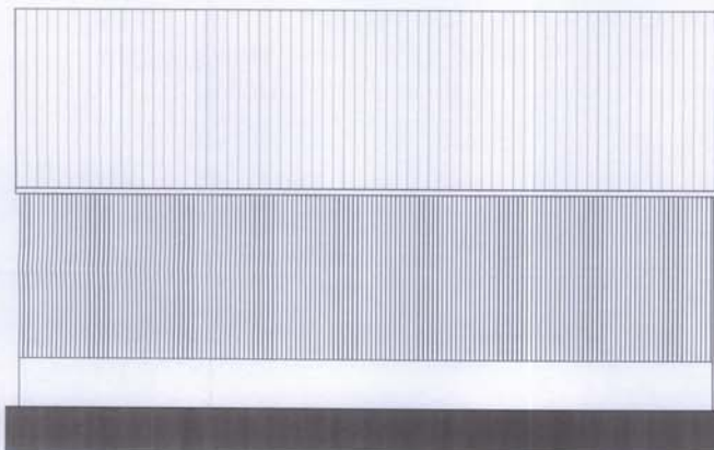
Proposed Dutch Barn Rear Elevation
